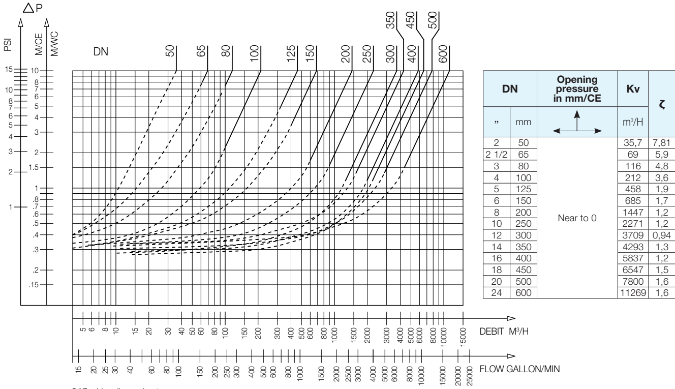
815 - Headloss chart
