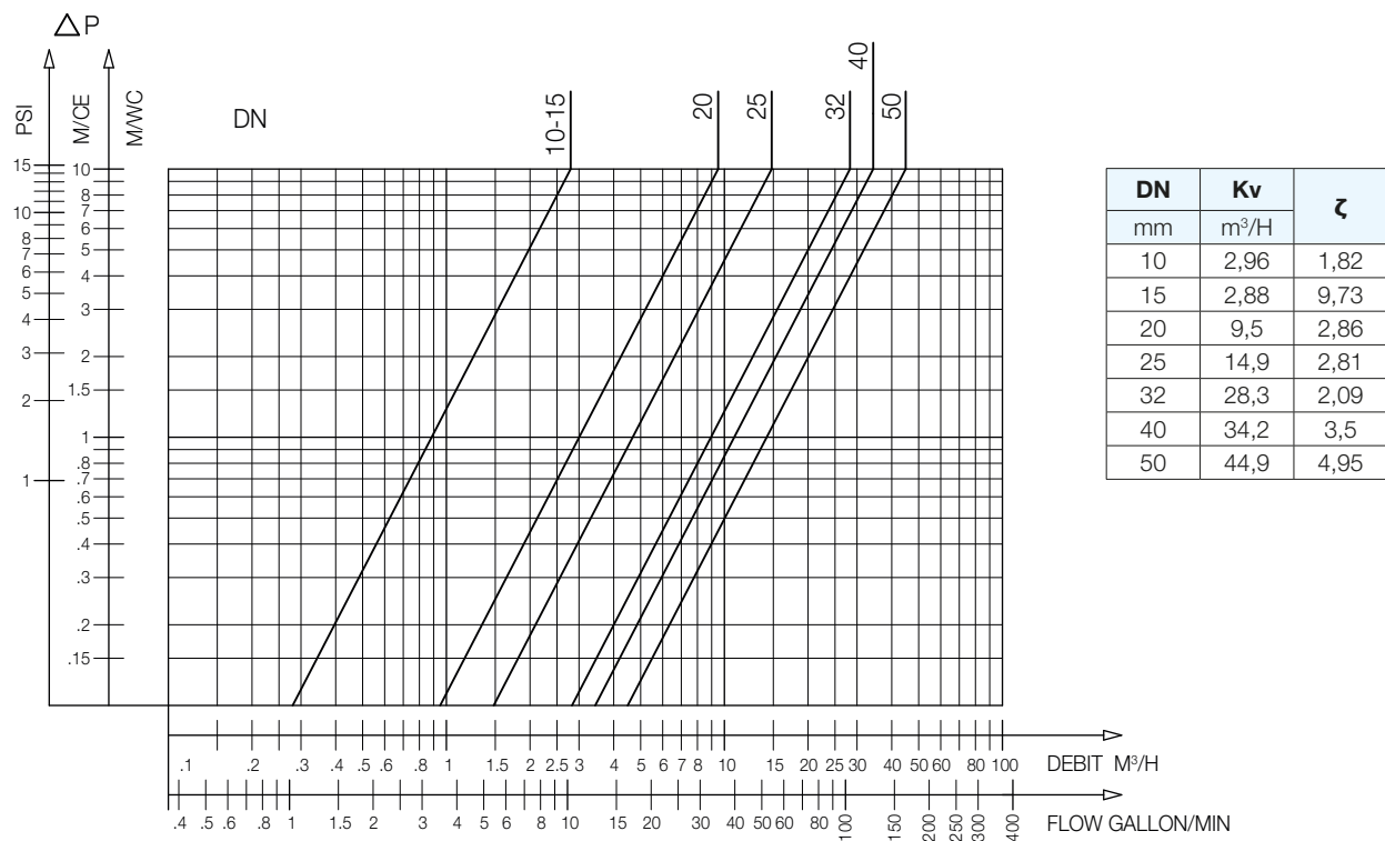
191D - Headloss chart
