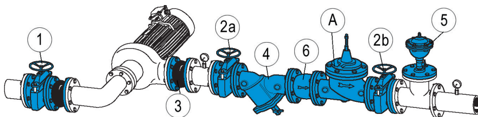
C 903 RB - Control valves installation diagram
